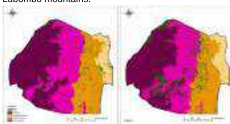
Figure 4: Baseline (left) and ecosystem assimilation.
