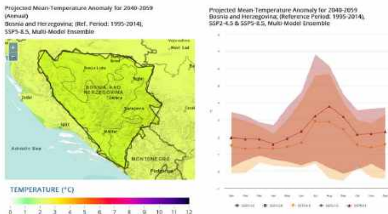
Figure 7: Projected Mean Temperature Anomaly for 2040-2059 in BiH compared to the reference period 1995-2014, SSP2-4.5 and SSP5-8.5, Multi-Model Ensemble. Source: CCKP.
