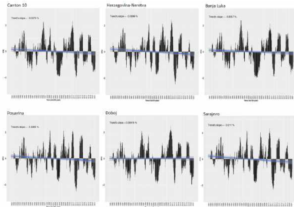
Figure 6: Monthly long term Drought index 29 (SPEI 18 months) for the Canton 10, Herzegovin-Nereta canton, Banja Luka region, Posavina canton, Dobo, region and Sarajevo canton for the period 1981-2021. Source: CHIRPS, TerraClimate.
