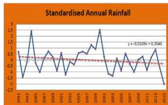
Figure 3: Standardised annual rainfall from 1981 to 2015
