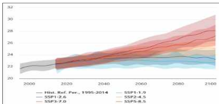
10. Figure 2: Multi-model ensemble mean temperature (°C) projections for Botswana.
